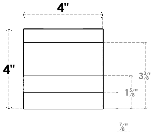
FRONT PROFILE
