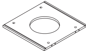
G-400X392mm(2pcs)
