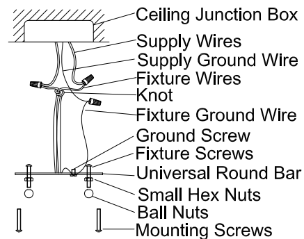
Wiring Drawing ( 2 )
