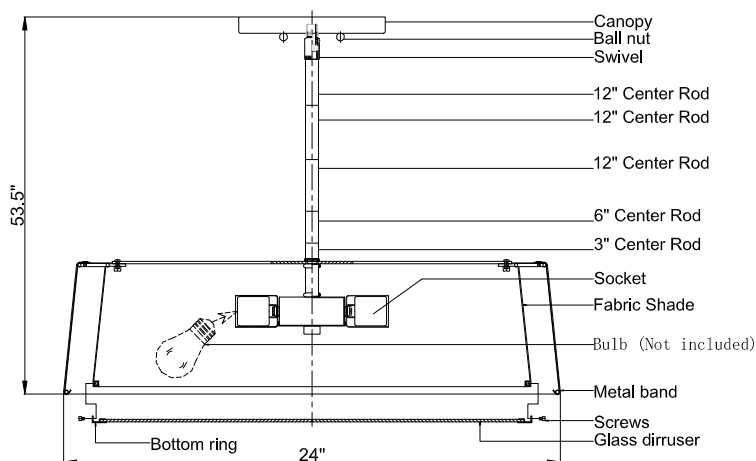
Brawing ( 1 )
