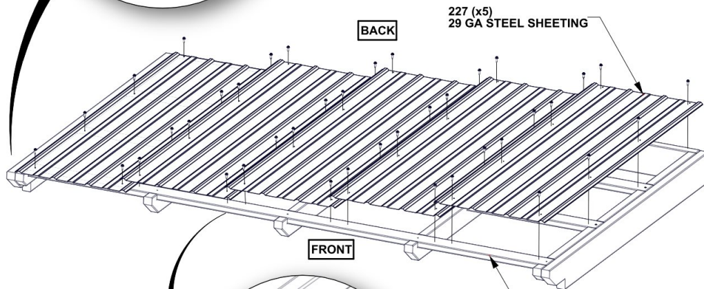
FLUSH EDGE OF SHEET WITH END OF RAFTER
