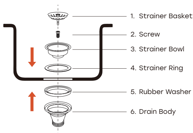
Basket Strainer Assembly Installation
