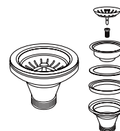
Basket Strainer
