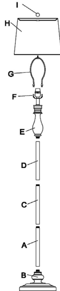
FLOOR LAMP
