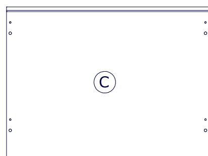
• CA2791 600x450x38mm
