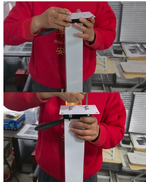
Step 2: Place the connecting piece on top of the flip piece and fix it with screw number 4
