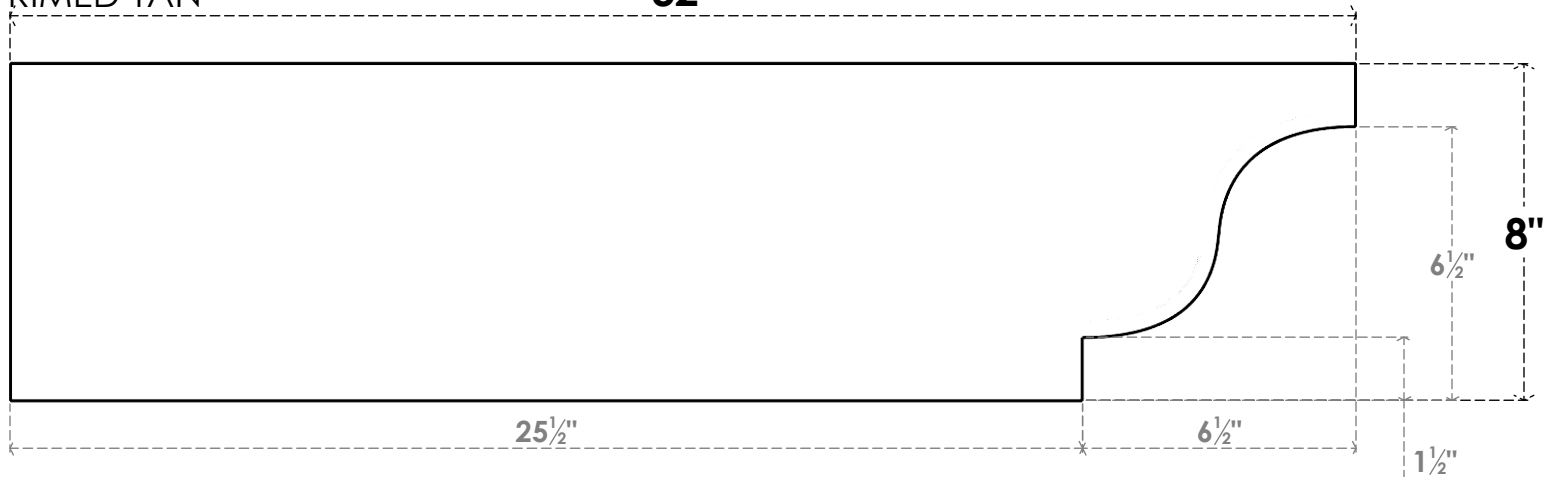
SIDE PROFILE
