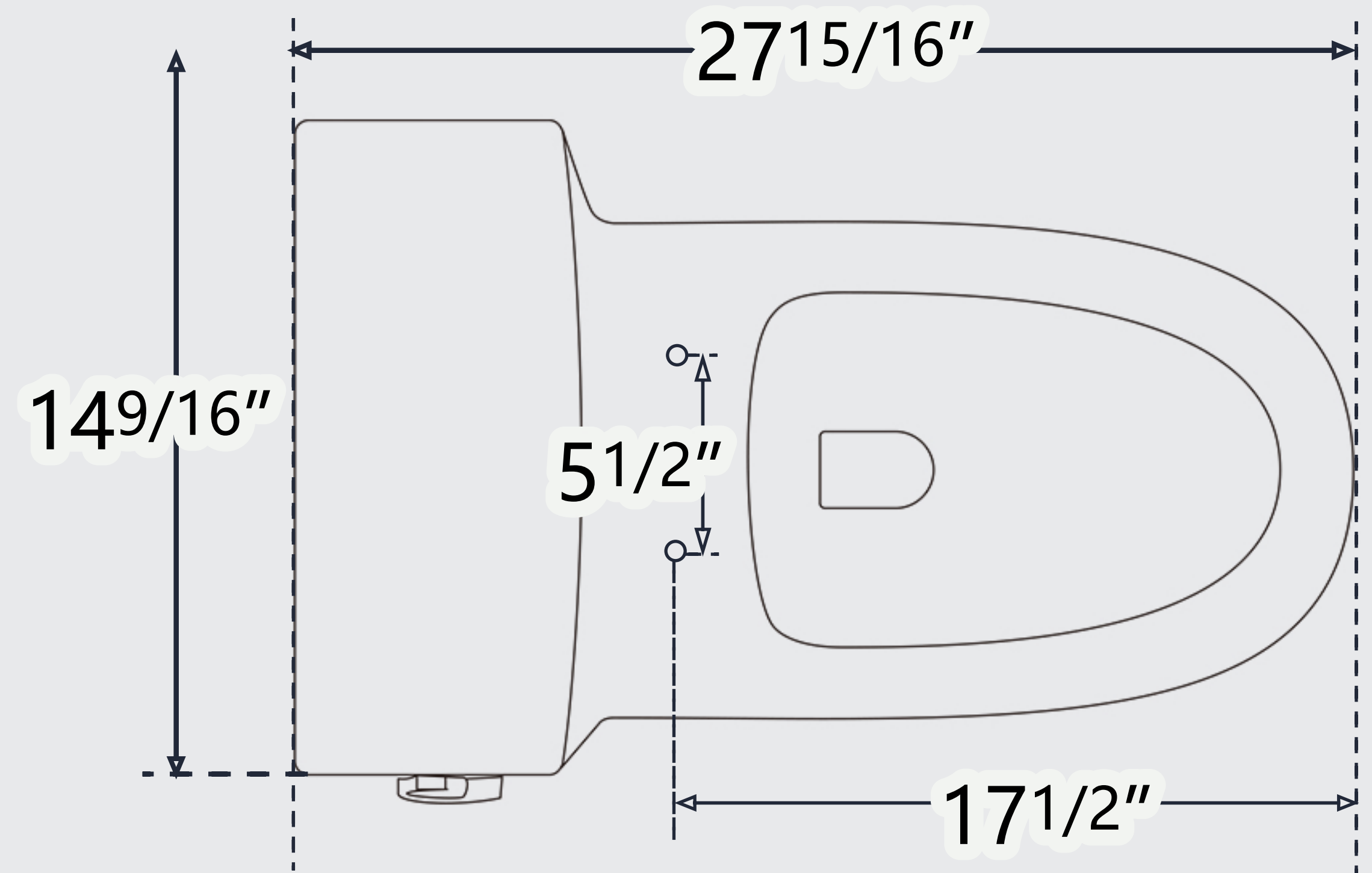
TOP VIEW
