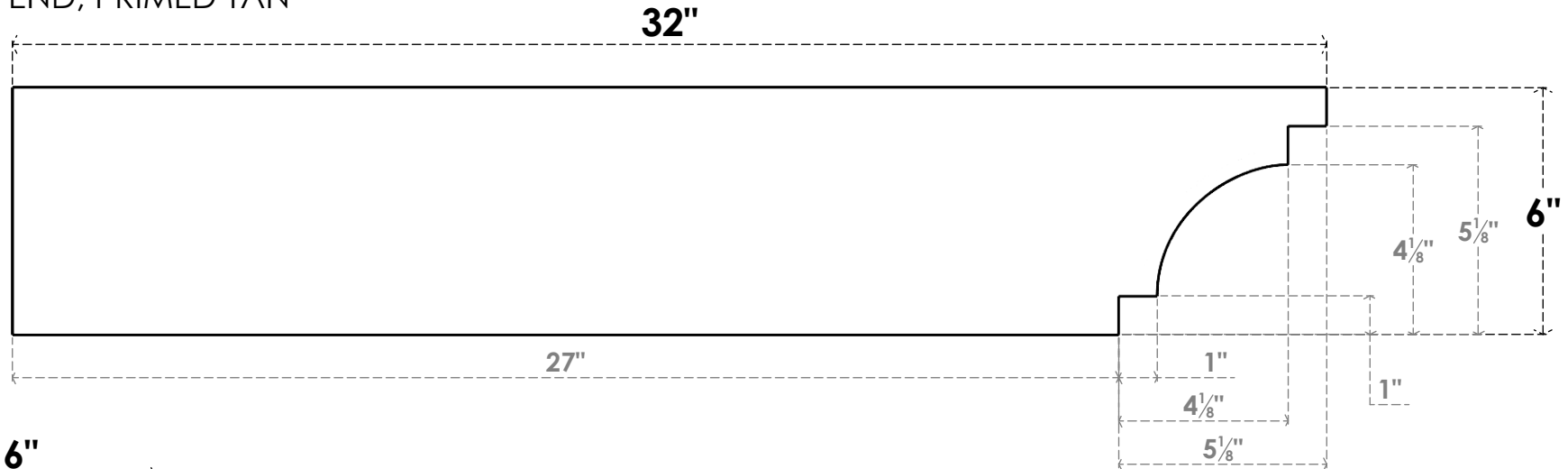
SIDE PROFILE
