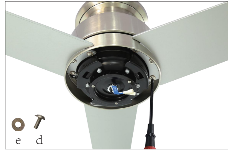
Step 7 Install the blade,tighten the screws.
