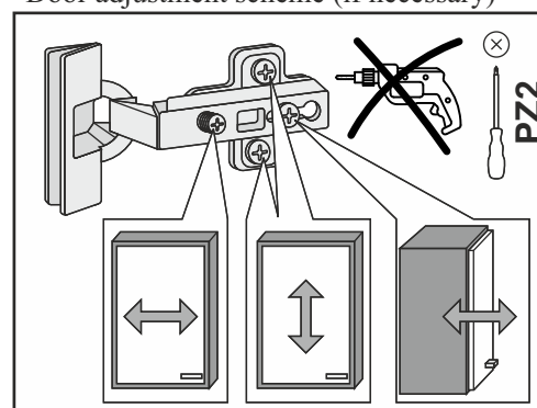
Türverstellschema (falls erforderlich) Door adjustment scheme (if necessary)
