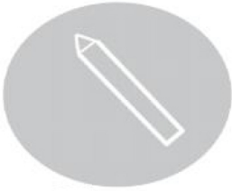
Oily pen
