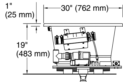
1-1/2" Bath Drain
