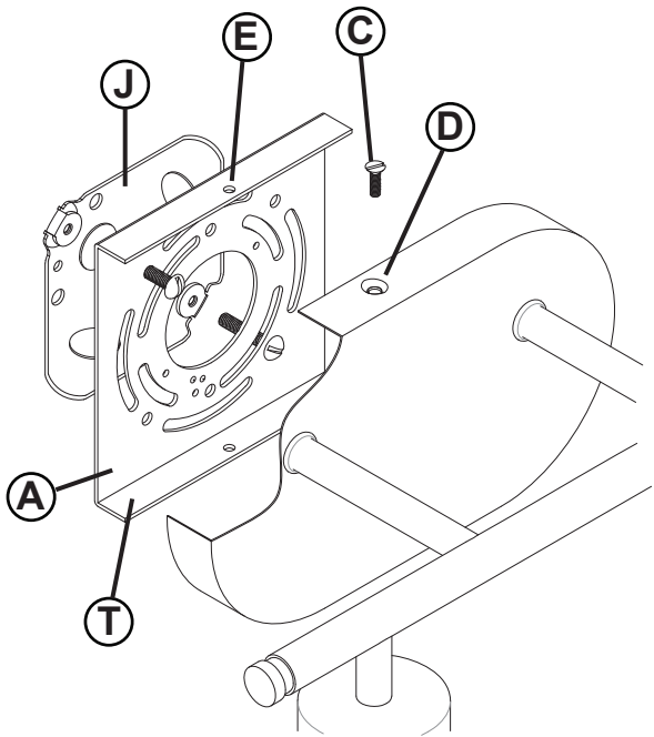
DRAWING 1 - GLASS INSTALLATION
