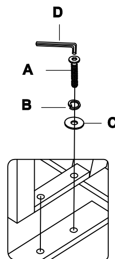
DETAIL A
