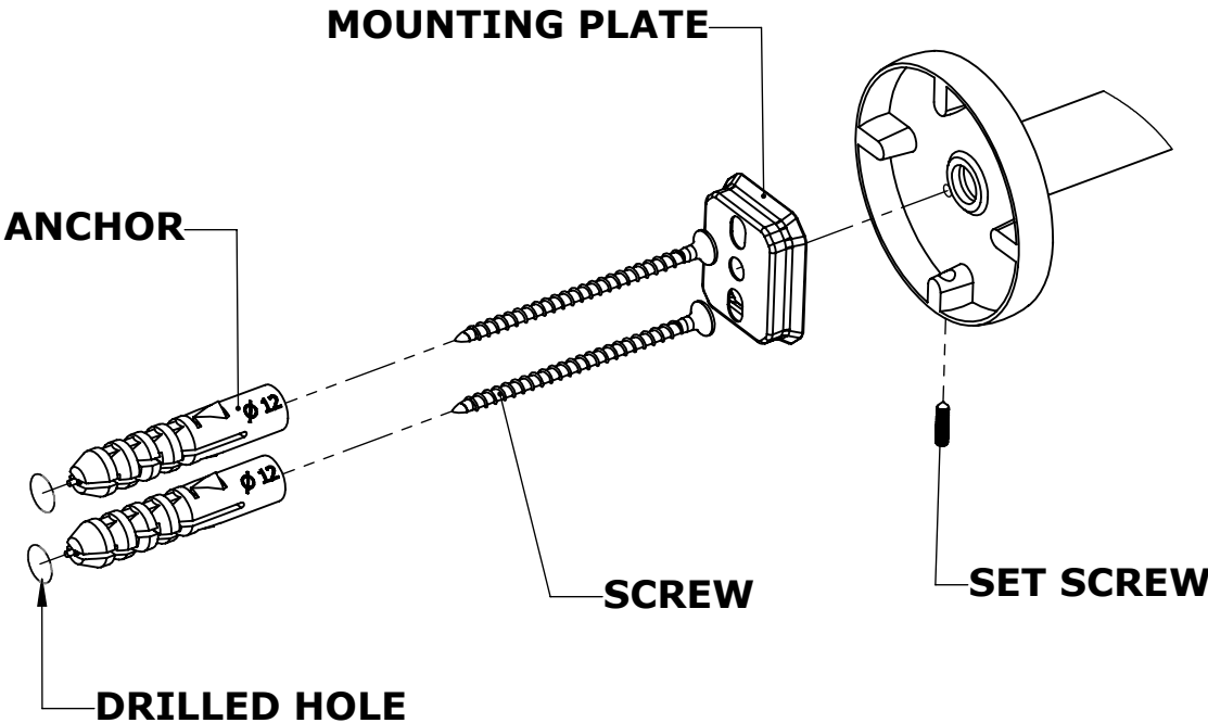
DETAIL M
