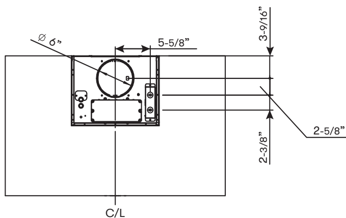
SIDE
