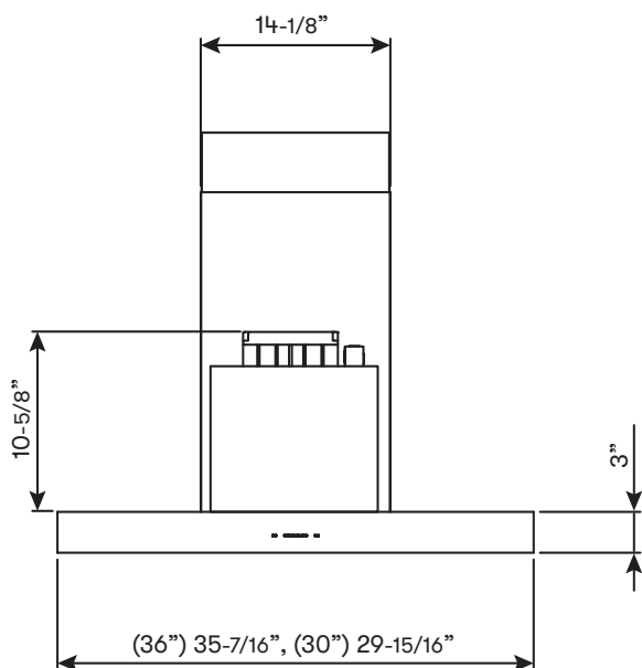
FRONT
