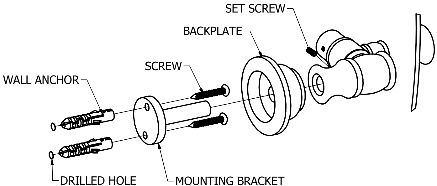
DETAIL A
