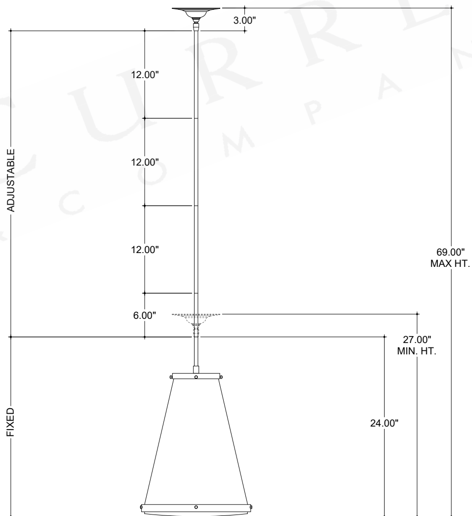
FRONT VIEW
