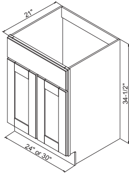
BT2421/3021 2 Doors
