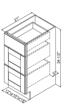
BT1221D/1521D/1821D 3 Drawers
