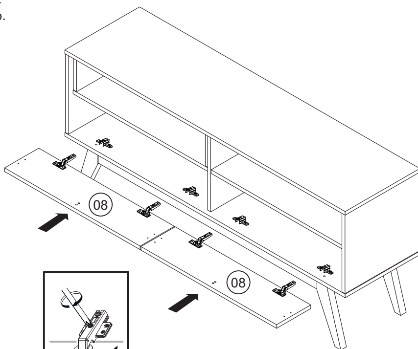
Horizontal Adjustment Ajuste Horizontal
