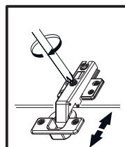
Horizontal Adjustment Ajuste Horizontal
