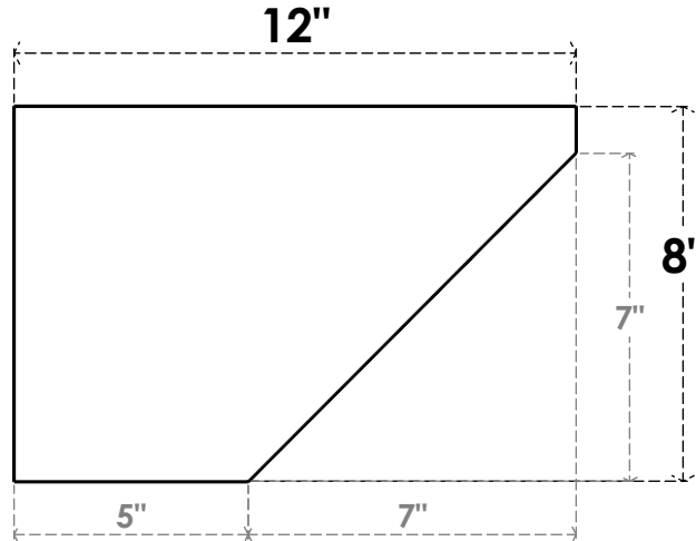
SIDE PROFILE
