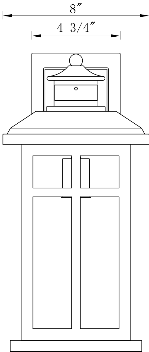
FRONT VIEW
