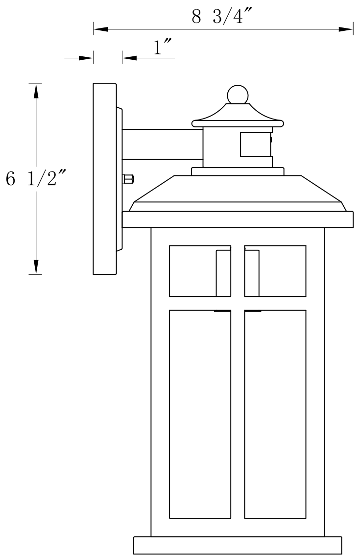
SIDE VIEW
