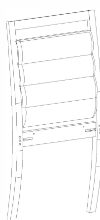
D3 (930x460x55mm) (36.61x18.61x2.16in)
