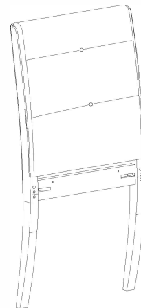
D4 (930x460x70mm) (36.61x18.61x2.75in)
