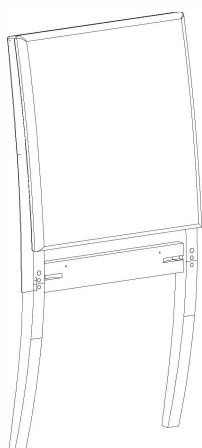
D (930x460x70mm) (36.61x18.61x2.75in)
