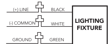
(Non-Dimming Wiring Diagram)
