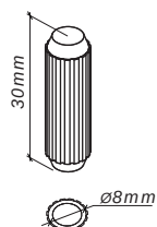
H1 x22
