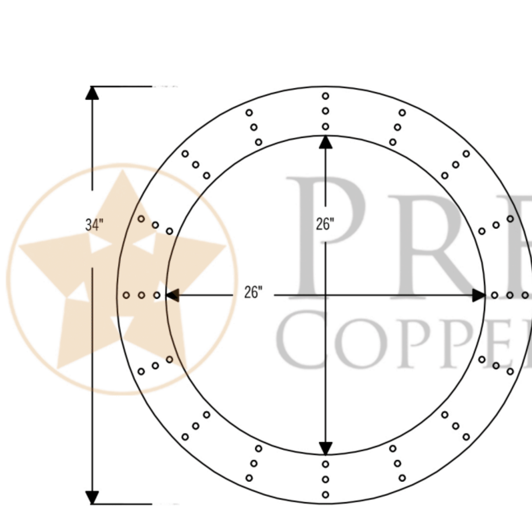
FRONT VIEW
