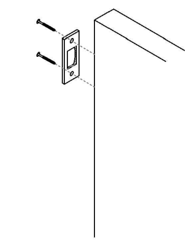
Step5:Install plastic tap to the side board
