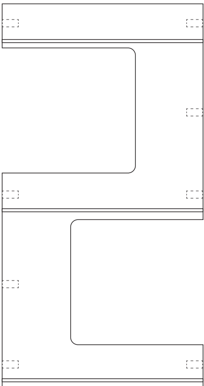
B-598x316x12mm(2pcs)
