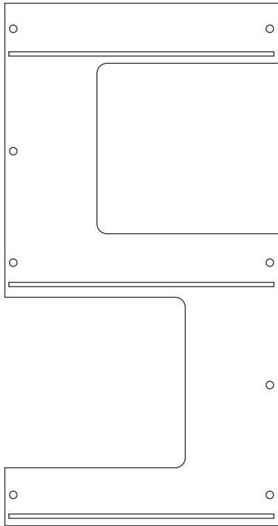
A-598x340x12mm(2pcs)
