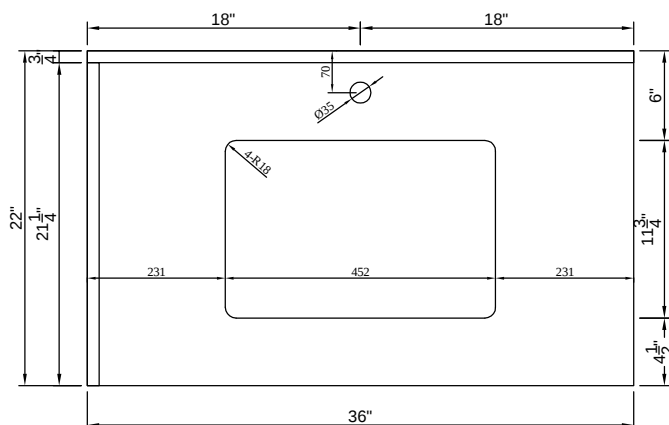
TOP VIEW OF VANITY CABINET
