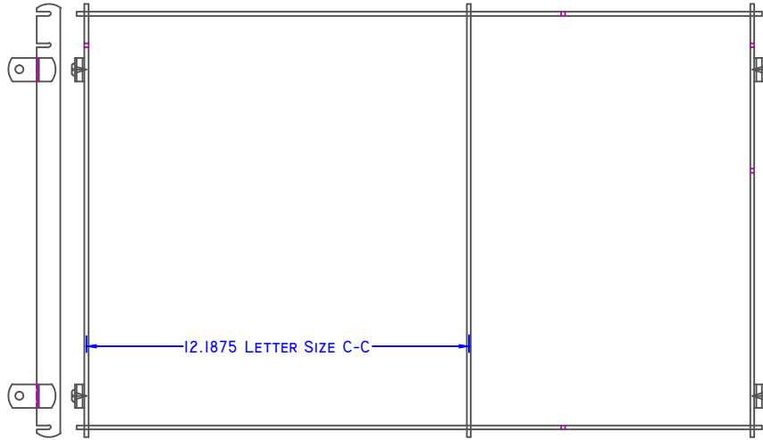
LETTER FILE HANGER ASSEMBLY (OPTION #2)
