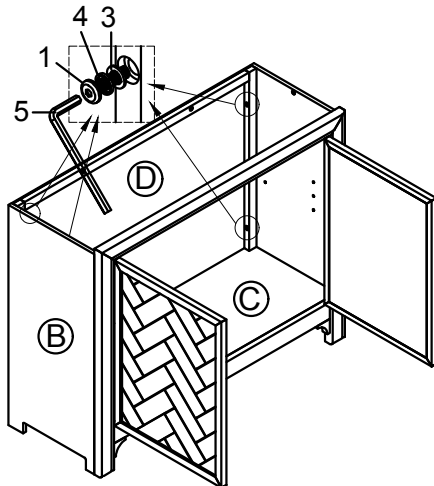
STEP 3: BACK FRAME: 4 POINT
