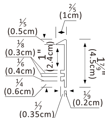
Aluminum section
