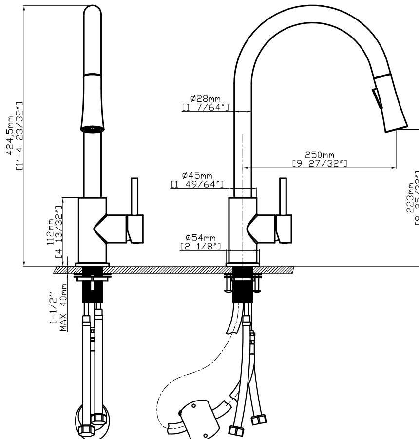
CRITICAL DIMENSIONS
