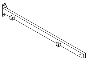
E Side Rail - Front
