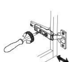
Depth adjustment
