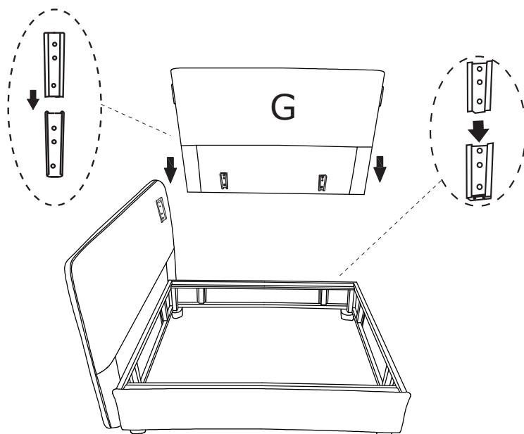
DIAGRAM 6 :Assemble th Armrest .
