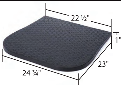
Tub Platform
