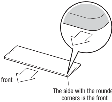
Upper Board (1)
