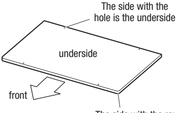
Lower Board (1)
