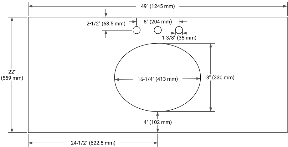
COUNTERTOP PLAN VIEW
