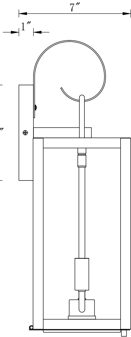
SIDE VIEW
