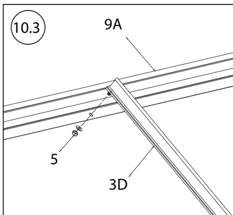
Attach the top end of Roof Rafter 3D to Roof Ridge Beam 9A using the uppermost Screw 5. Repeat 3X.
