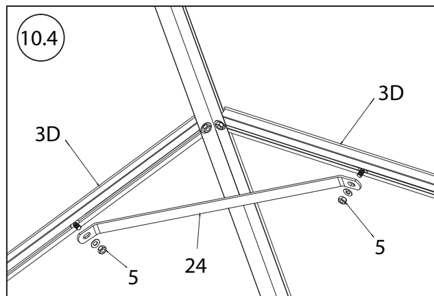
Attach Roof Brace 24 to Roof Rafter 3D using the second Screw 5. Repeat 1X.
