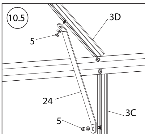
Attach Roof Brace 24 to Sidewall Vertical Support 3C using the next lowest Screw 5 on Roof Rafter 3D and the second Screw 5 on 3C. Repeat 3X.
