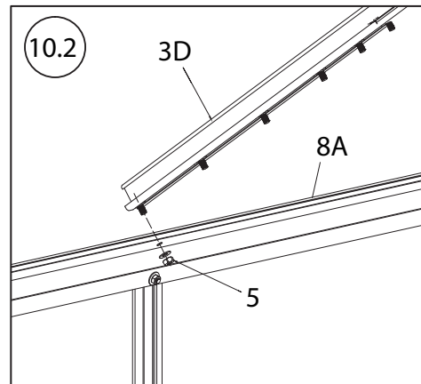
Attach the lower end of Roof Rafter 3D to Sidewall Horizontal Beam 8A using the lowermost Screw 5. Repeat 3X.
