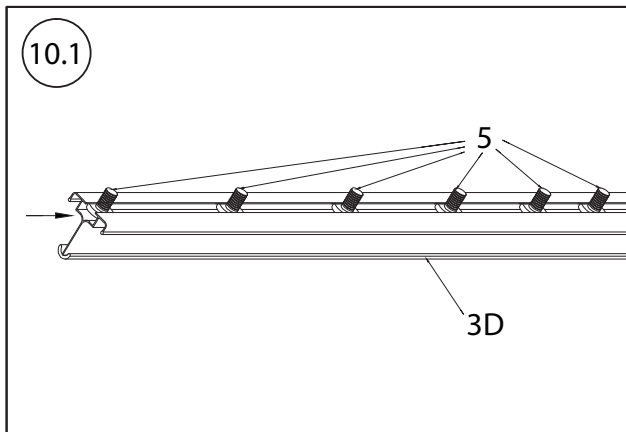
Slide (6) Screw 5 into the channel on (4) Roof Rafter 3D.
