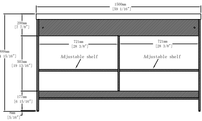
Back View
