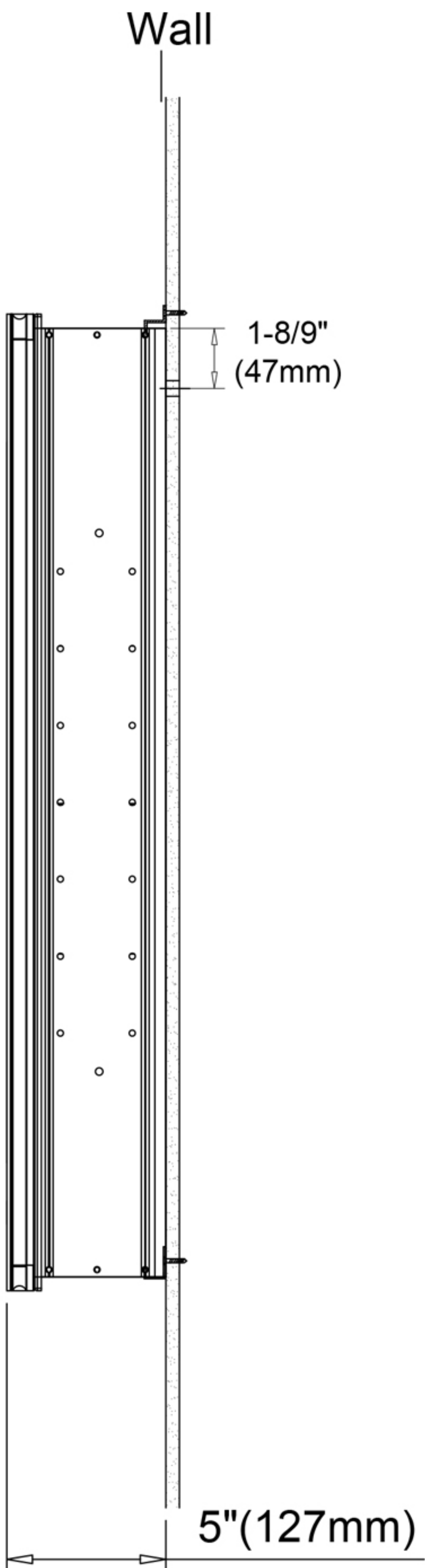
Surface Mount
