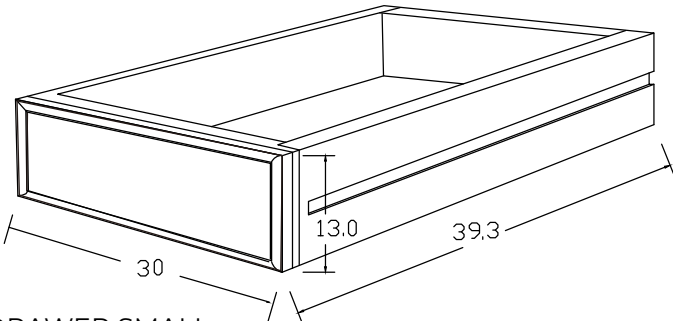
DETAIL DRAWER SMALL
