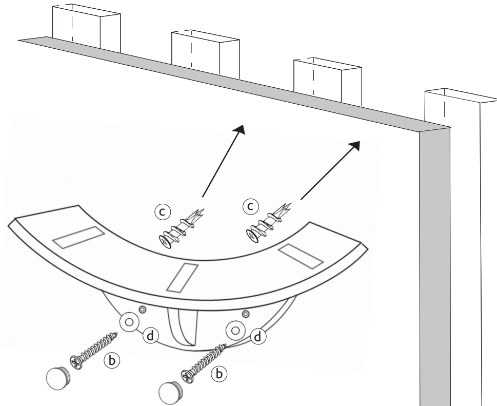
Drywall connection
