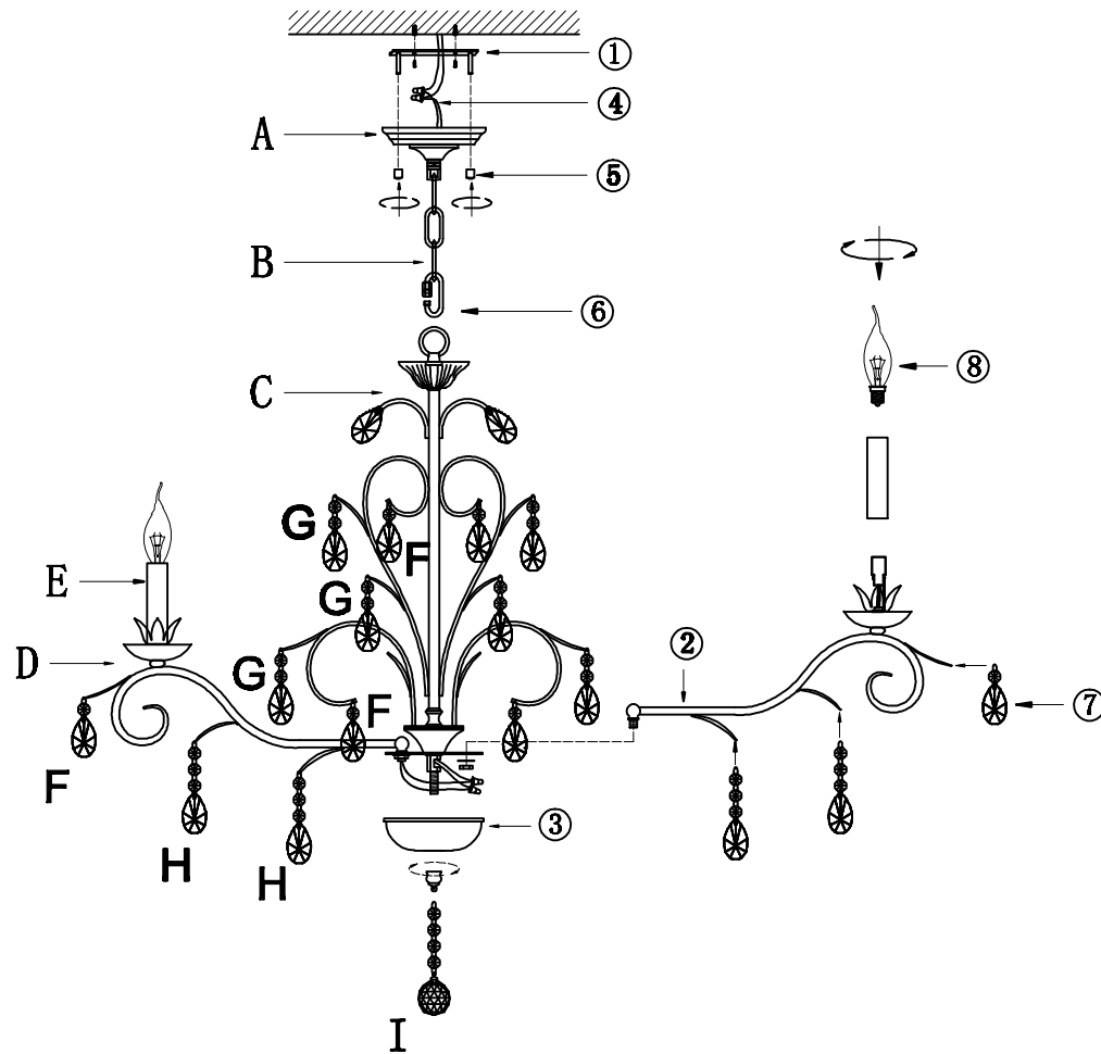
Installation sequence diagram
