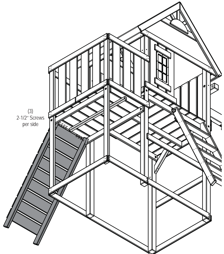
Underdeck View
