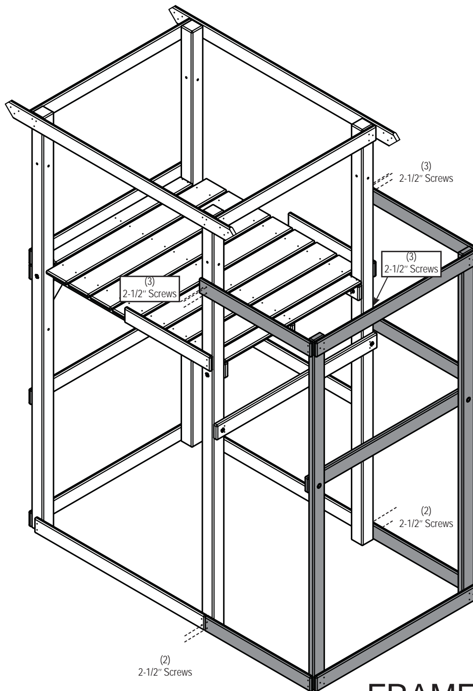
FRAME C
